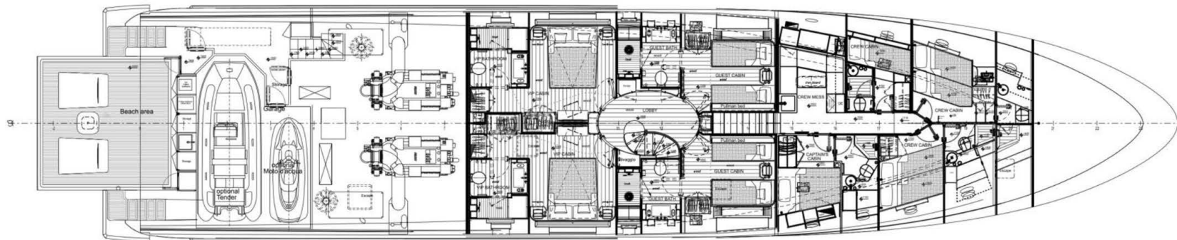
Lower deck
