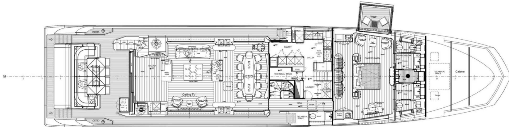
Main deck
